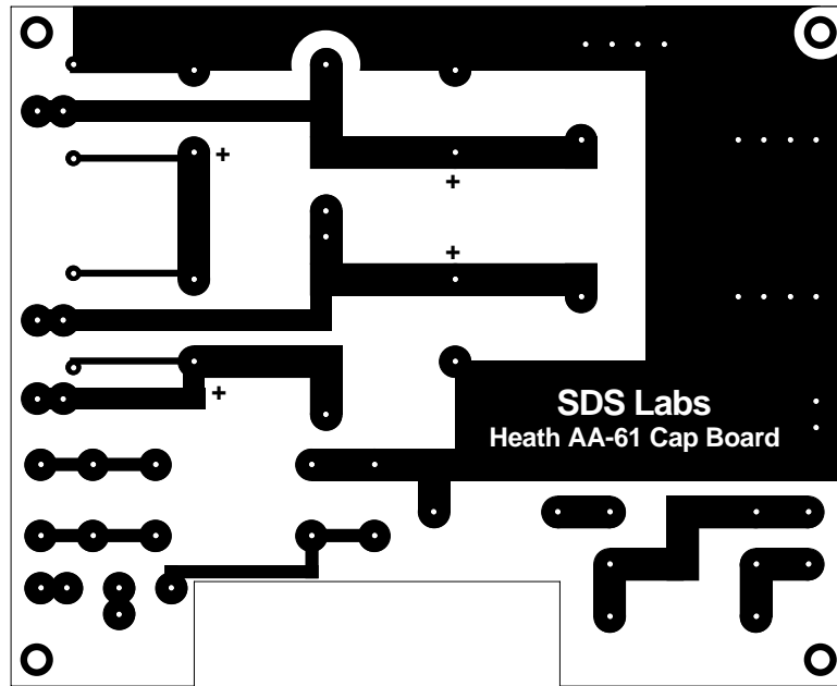
Capacitor Board Layout
