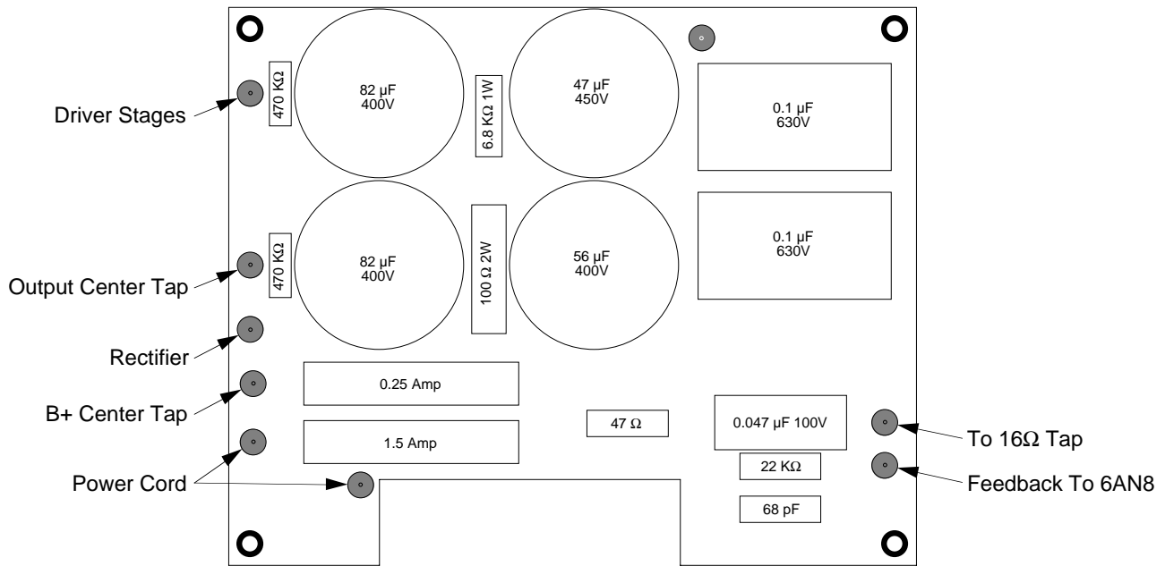
Capacitor Board Parts Placement and Wiring
