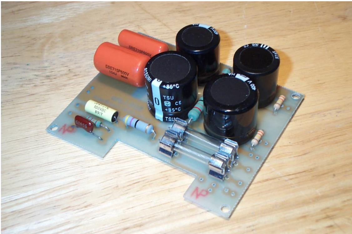
Heath UA-1 (UA-2 or AA-61) Power Supply Capacitor Board
